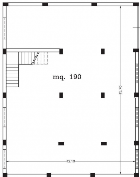
PIANO SEMINTERRATO rapp. 1:100
